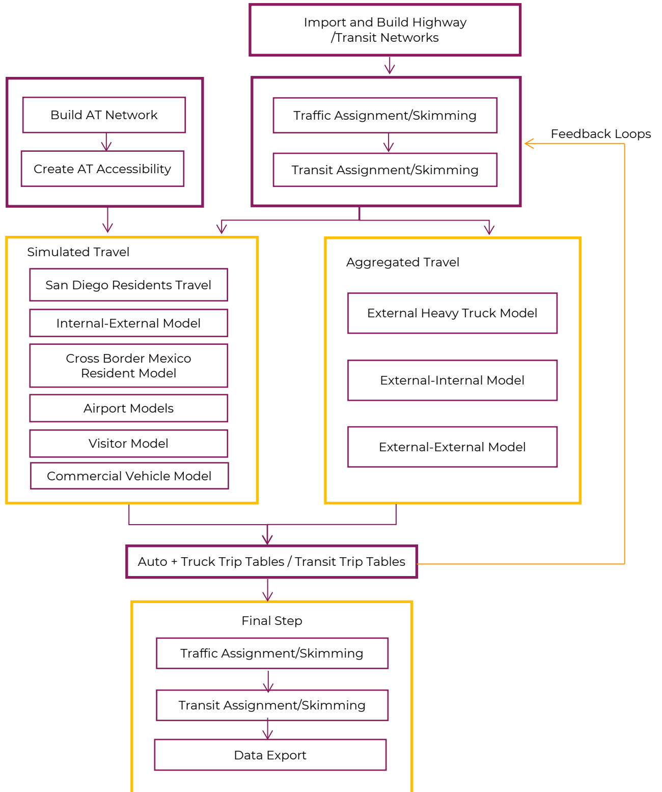
Figure F-2: SANDAG ABM2+ Flow Chart
