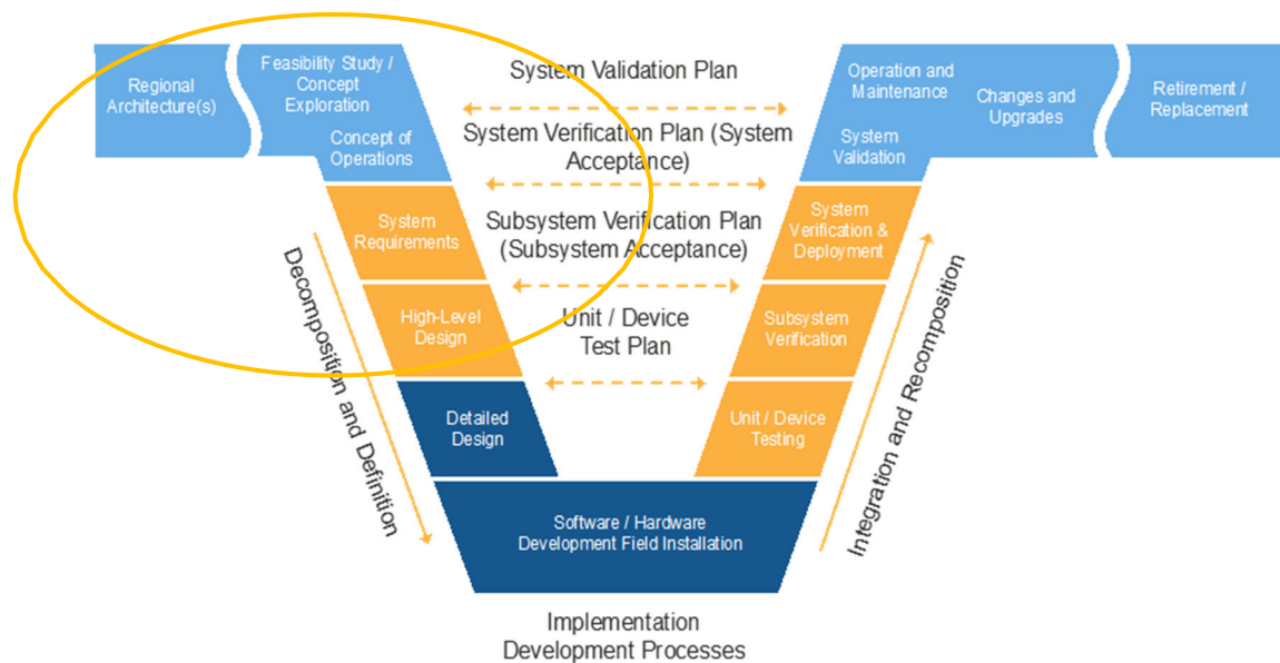
Figure 19: FHWA V-Diagram Systems Engineering Process Model
